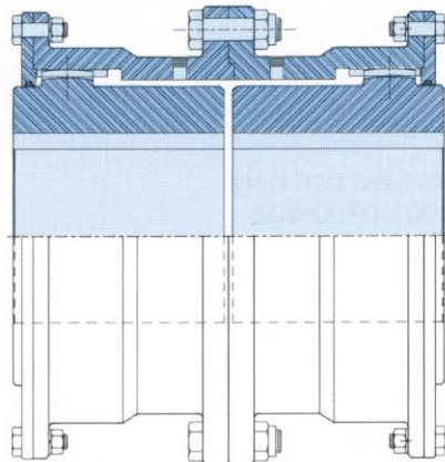
Heavy Duty
