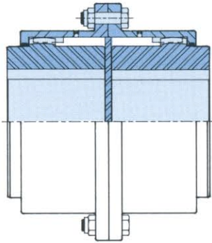
Limited End Float Full-Flex
