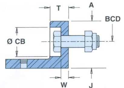
Shrouded Bolt
