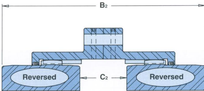
Both Hubs Reversed
