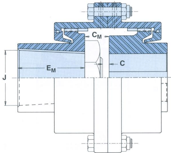
Full-Flex
