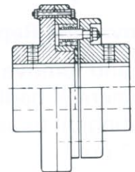
Shear Pin
