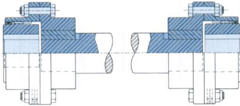
Tandem — Rigid halves on floating shaft Maximized offset capacity
