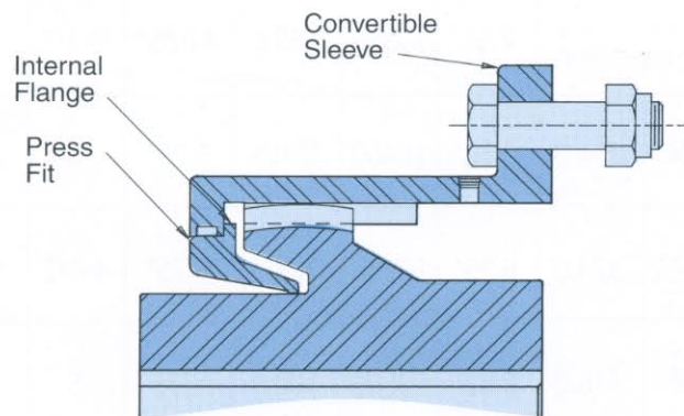
Metal Seal
