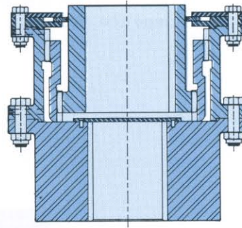
Heavy Duty Vertical Full-Flex
