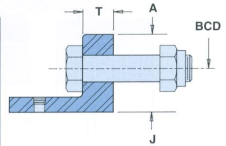
Exposed Bolt
