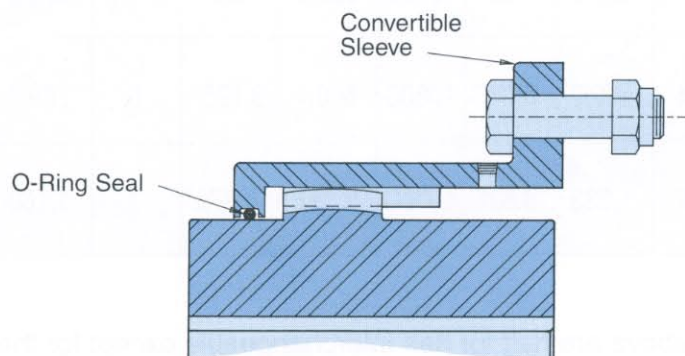
O-Ring Seal
