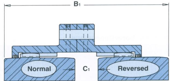
One Hub Reversed
