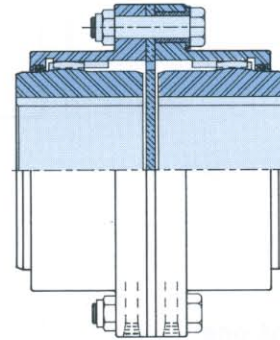
Insulated Full-Flex
