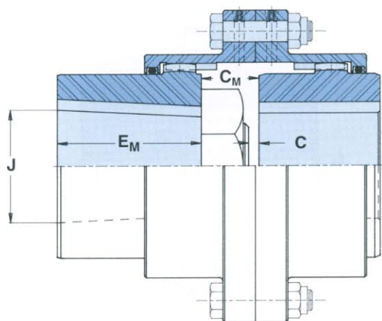
Full-Flex
